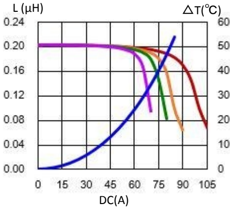
4. CDEPH7212NP-R20LC
