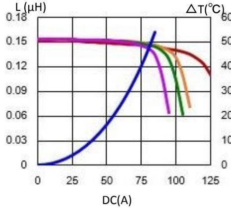
2. CDEPH7212NP-R15LC
