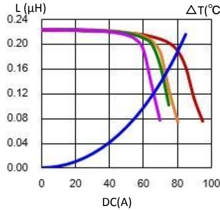
5. CDEPH7212NP-R22LC
