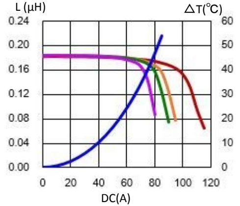
3. CDEPH7212NP-R18LC
