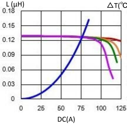
1. CDEPH7212NP-R13LC
