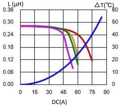
6. CDEPH7212NP-R28LC
