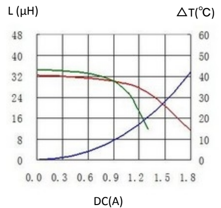
9. CDRH6D38T125NP-330PC
