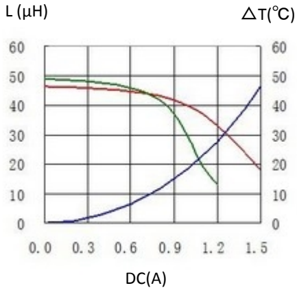
10. CDRH6D38T125NP-470PC
