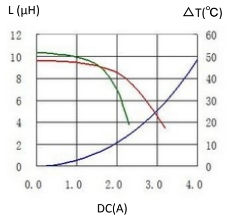
6. CDRH6D38T125NP-100PC
