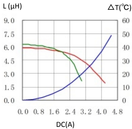
4. CDRH6D38T125NP-5R6NC
