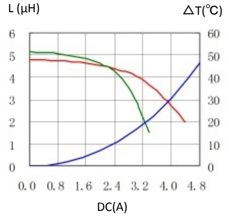
3. CDRH6D38T125NP-4R7NC
