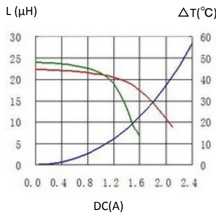
8. CDRH6D38T125NP-220PC
