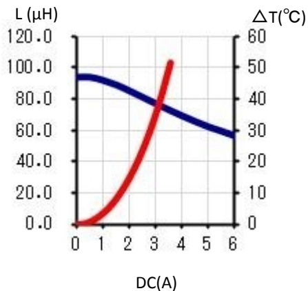
20. CY1260AT125DS-820MC
