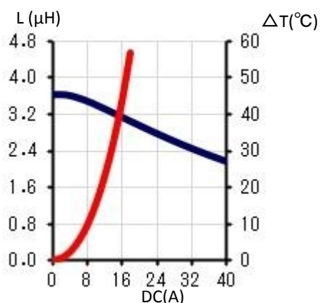
7. CY1260AT125DS-3R3MC
