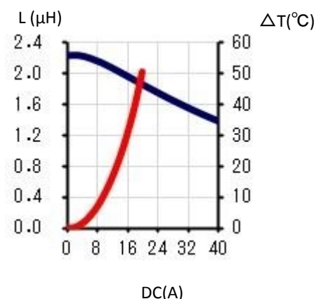
6. CY1260AT125DS-2R2MC
