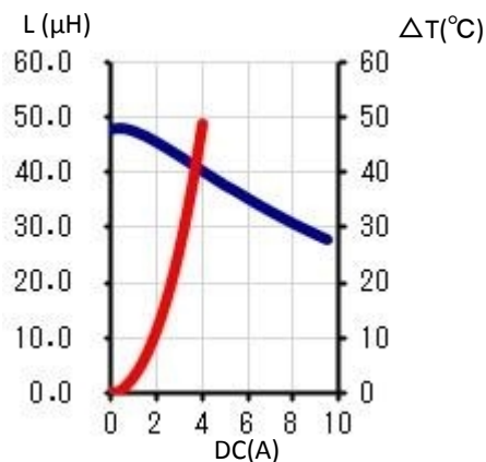
18. CY1260AT125DS-470MC
