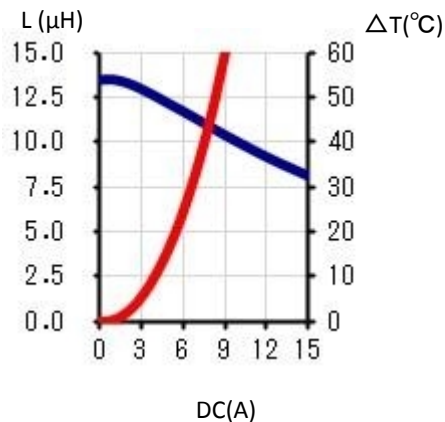
12. CY1260AT125DS-120MC
