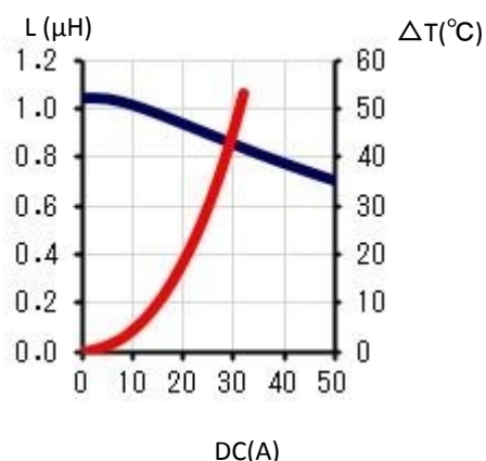
4. CY1260AT125DS-1R0MC
